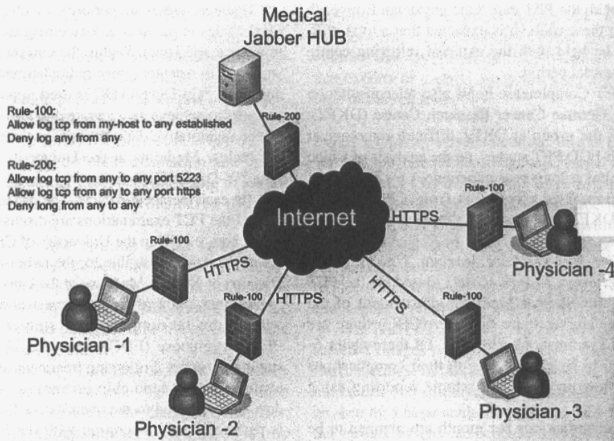
Figure 8. Jabber network.
