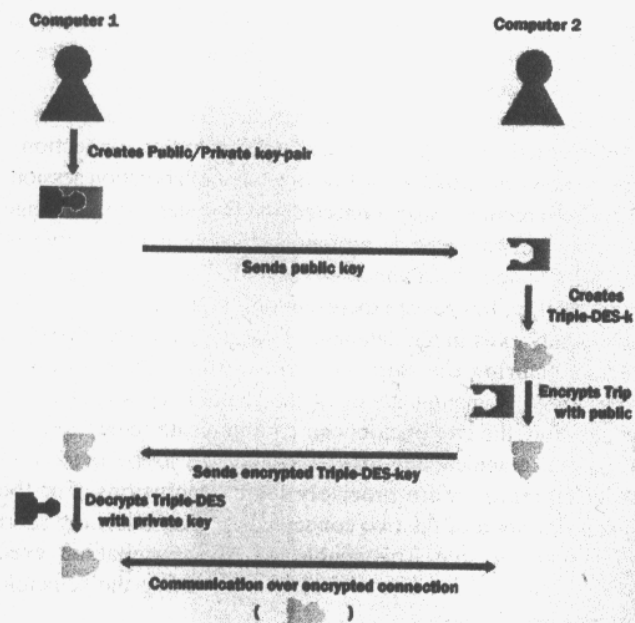
Figure 6. Encrypted connection.
